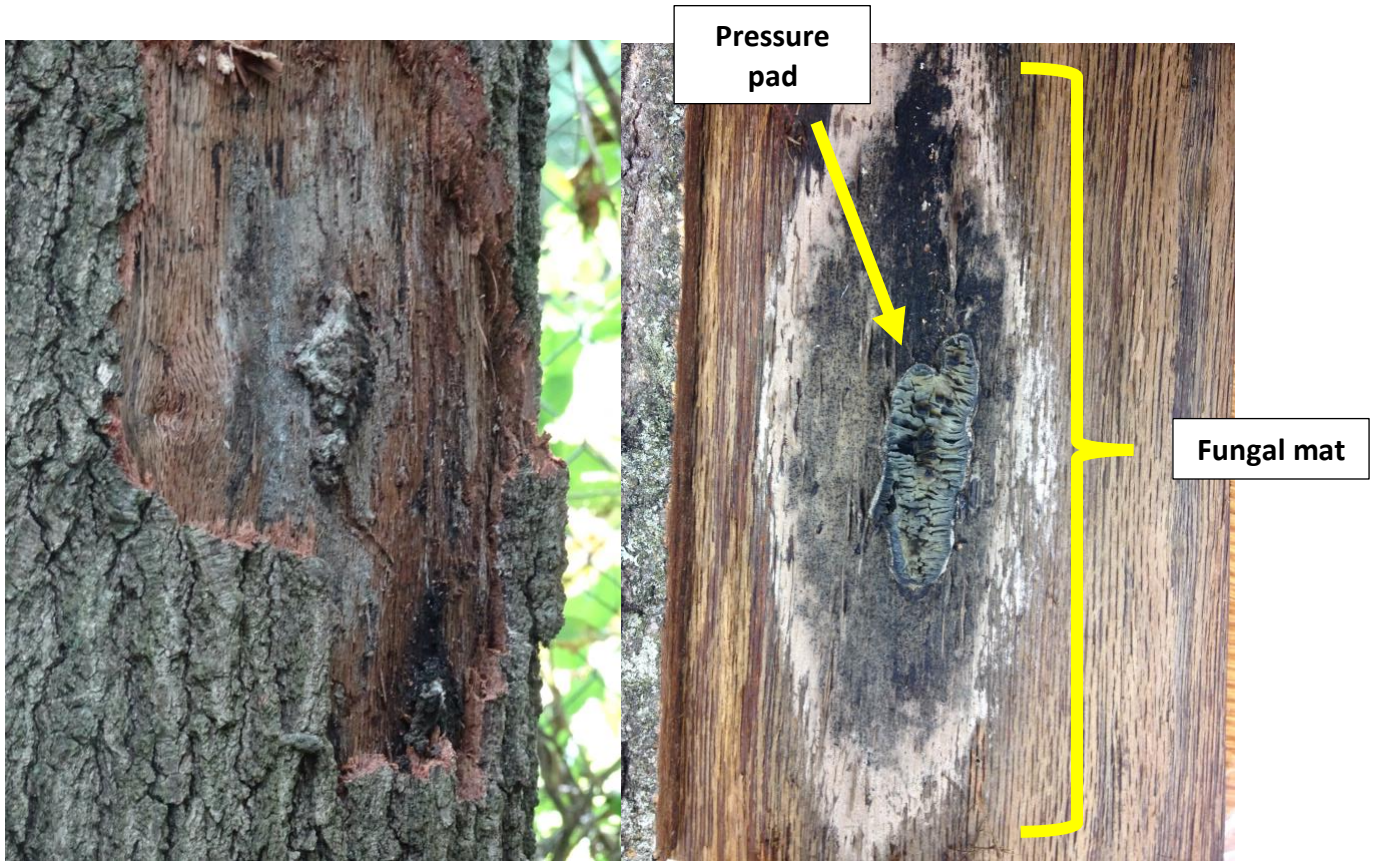
Fungal mats and pressure pads growing on dead red oak tree. Credit: Invasive Species Centre
